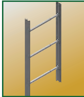
Heavy Duty Vertical Shore with three cylinders
